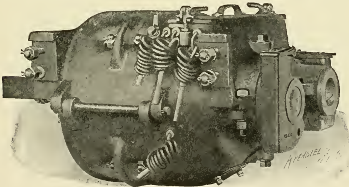
Fig. 31. Westinghouse Railway Motor—Commutator End
